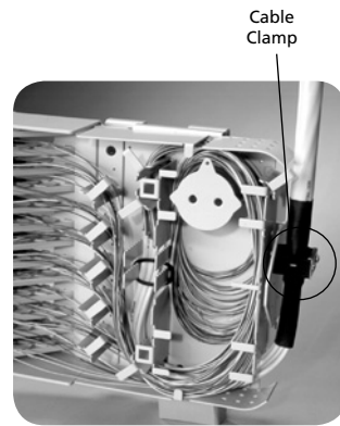
72-Position FTB Loaded with Multifiber Breakout Cable
